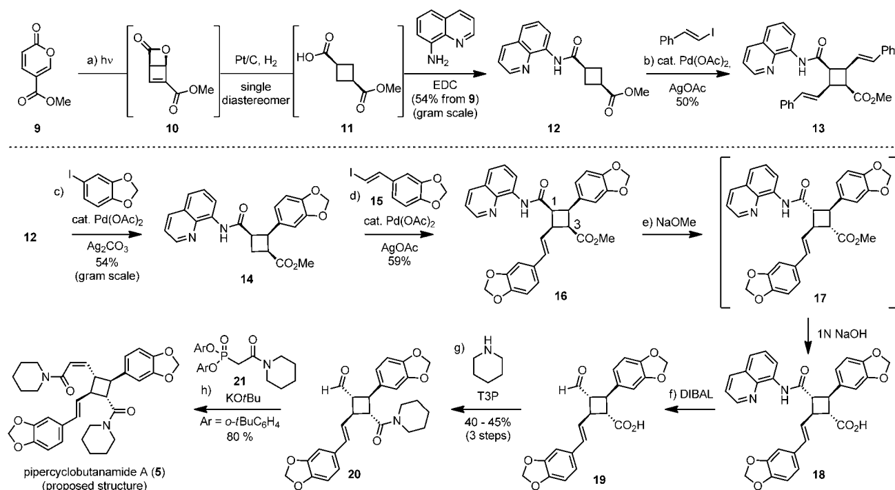
Scheme 1. Total synthesis of the proposed structure of pipericyclobutanamide A ( 5 ). Reagents and conditions: a) 450-W Hanovia lamp, Pyrex filter, CH 2 Cl 2 , 15°C, 96 h; then H 2 , Pt/C, 4 h; then 8-aminoquinoline (1.2 equiv), EDC (1.2 equiv), 0 to 23°C, 3 h, 54%. b) (2-iodovinyl)benzene (3.0 equiv), Pd(OAc) 2 (0.15 equiv), AgOAc (3.0 equiv), PhMe, 80°C, 12 h, 50%. c) Pd(OAc) 2 (0.15 equiv), Ag 2 CO 3 (1.0 equiv), PivOH (1.0 equiv), 1-iodo-3,4-methylenedioxybenzene (2.0 equiv), t BuOH, 85°C, 15 h, 54%. d) 15 (2 equiv), Pd(OAc) 2 (0.15 equiv), AgOAc (1.5 equiv), PhMe, 80°C, 10 h, 59%. e) NaOMe (2.0 equiv), MeOH/THF (1:4), 45°C, 2 h, then 1 N NaOH, 1 h. f) DIBAL (3.5 equiv), THF, –78°C, 0.5 h. g) piperidine (3.0 equiv), T3P (1.5 equiv), CH 2 Cl 2 , 23°C, 15 min, 40–45% (3 steps). h) 21 (1.5 equiv), KOtBu (1.5 equiv), THF, –78°C to 0°C, 2 h, 80%. DIBAL = diisobutylaluminum hydride, EDC = 1-ethyl-3-(3-dimethylaminopropyl)carbodiimide, T3P = propylphosphonic anhydride, THF = tetrahydrofuran.
